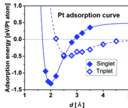
Pt-graphene complex
