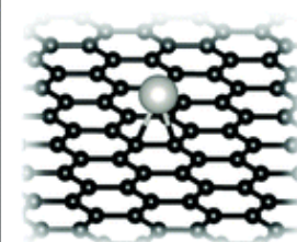
Pt-graphene complex
