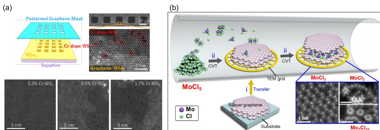
Figure 1 (a) Selective area Cr doping of WS 2 using a prepatterned graphene mask. The doping concentration can be controlled by adjusting the reaction time. (b) Intercalation of bilayer graphene using MoCl 5 as a precursor via gas-phase reaction. The resulting intercalated structures were identified as MoCl 3 networks, MoCl 2 chains, and Mo 5 Cl 10 rings, rather than a MoCl 5 lattice.
