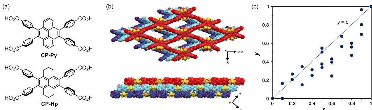
Figure 1. Non-stoichiometric co-crystalline frameworks formed through 2D hydrogen-bonded networking of CP-Py and CP-Hp . (a) Molecular structure of the components. (b) Crystal structure of the co-crystalline framework, where yellow-colored parts denote disordered moieties of CP-Py and CP-Hp . (c) Composition in single-crystals of CP-HpPy-1 ( x, y ), where x and y denote the molar fraction and occupancy of CP-Hp in the initial solution and the resultant single crystal, respectively.
