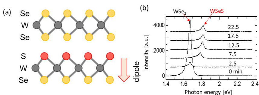
Figure 1 Fabrication of Janus TMD. (a) Typical structure of (top) normal TMD ( \text{WSe}_2 ) and (bottom) Janus TMD ( \text{WSeS} ). (b) Time profile of PL spectra during Janus TMD ( \text{WSeS} ) formation obtained with in-situ monitoring plasma functionalization.
