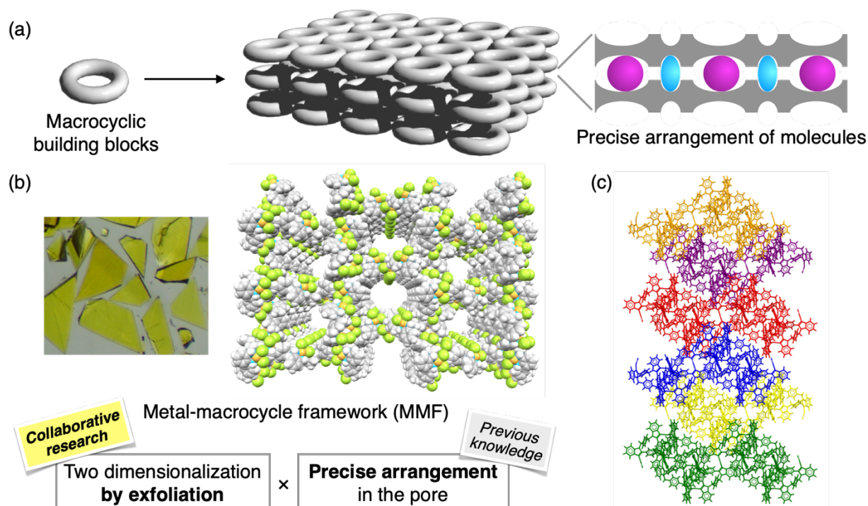
Figure 1 (a) Schematic of the basic concept of this work. (b) Structure of a porous crystal, metal-macrocycle framework, and its application for 2.5-dimensional materials. (c) Structure of a 2D-MOF with bumpy interlayer nanospaces.
