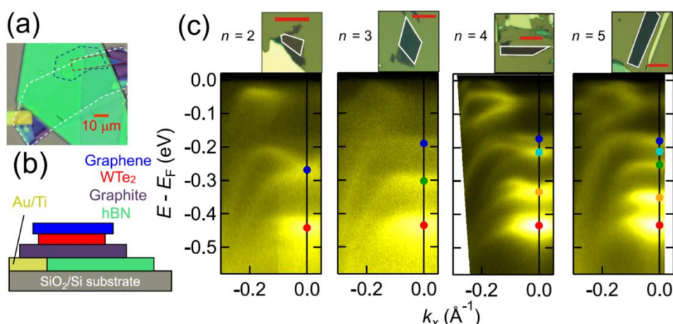
Figure 1 (a) Optical microscope image of the fabricated graphene/ \text{WTe}_2 /graphite/h-BN heterostructure sample. (b) Schematic of the fabricated sample. (c) Upper panels: The optical microscope images of the 2–5-layer \text{WTe}_2 flakes (white frames) used for ARPES. The red bars represent the 10-mm length. Lower panels: Obtained ARPES images for 2–5-layer \text{WTe}_2 . The makers (•) indicate the positions of the intensity peaks at k_x = 0 .
