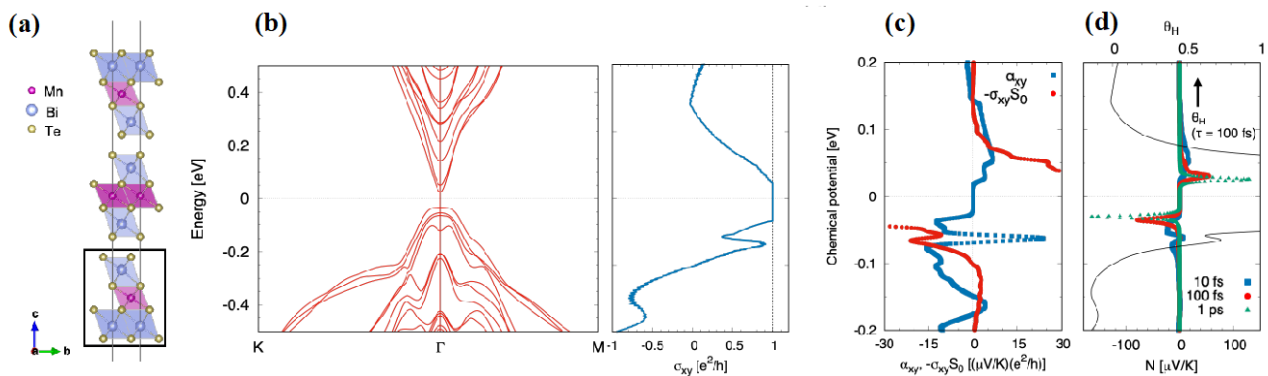
Figure 1 (a) The structure of \text{MnBi}_2\text{Te}_4 three septuple layers (3SLs). The lined areas indicate a septuple layer. (b) Electronic band structure and the chemical-potential dependence of anomalous Hall conductivity of \text{MnBi}_2\text{Te}_4 with 3SLs. (c) The transverse thermoelectric conductivity and Seebeck-induced term of \text{MnBi}_2\text{Te}_4 with 3SLs. (d) Calculated anomalous Nernst coefficient and Hall angle ratio with different constant relaxations for \text{MnBi}_2\text{Te}_4 with 3SLs.
