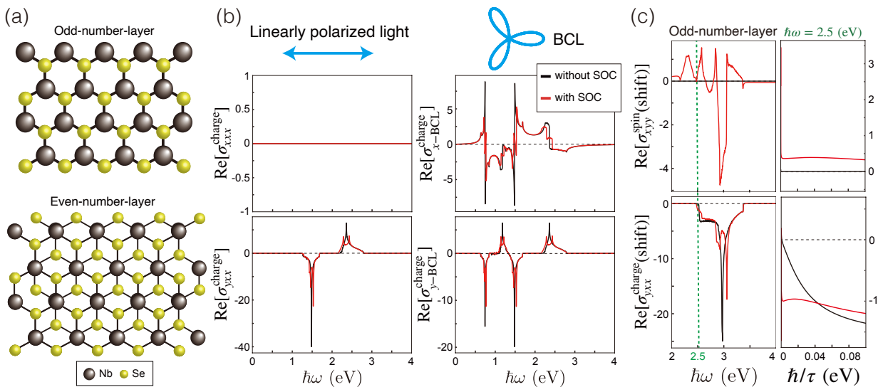
Figure 1 (a) Crystal structure of few-layered NbSe 2 . (b) Nonlinear optical conductivities of monolayer NbSe 2 for SHG process (left) and incident BCL (right). (c) Spin and charge shift-current conductivities of monolayer NbSe 2 and the dependence of relaxation time \tau .
