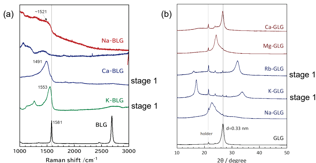
Figure 1 The products of vapor phase intercalations of bi-layer graphene (BLG) and graphene like graphite (GLG). (a) Raman spectra of intercalated BLGs. (b) XRD patterns of intercalated GLGs.
