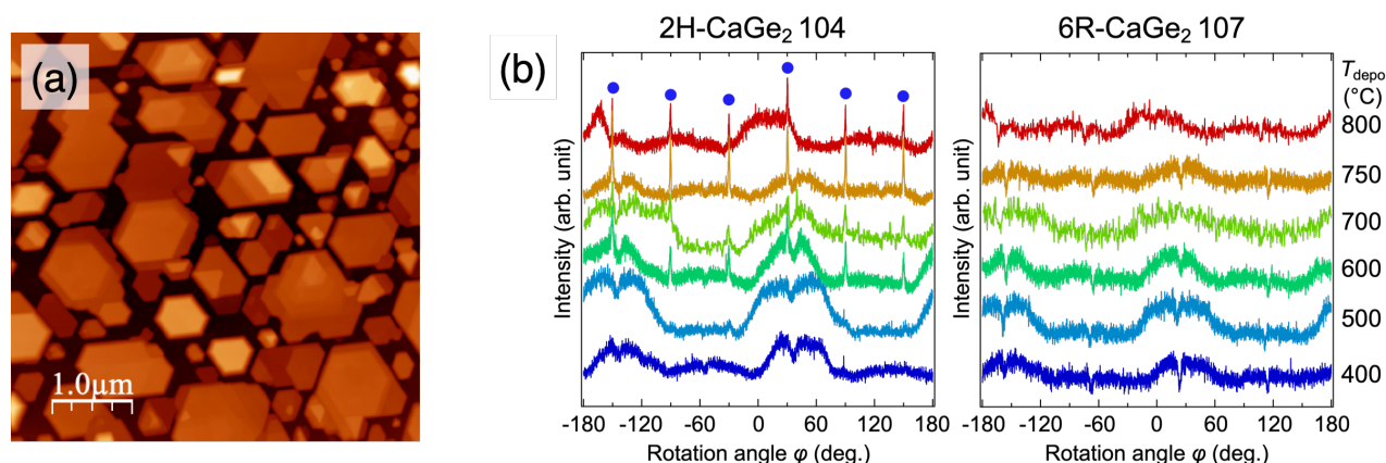
Figure 1 (a) Atomic force image of \text{CaGe}_2 films on FZ-Si(111) substrates grown by molecular beam epitaxy at 800 °C. (b) X-ray diffraction \phi -scan of the 2H 104 and the 6R 107 obtained from the \text{CaGe}_2 films grown at different deposition temperatures ( T_{\text{depo}} = 400\text{--}800 °C).
