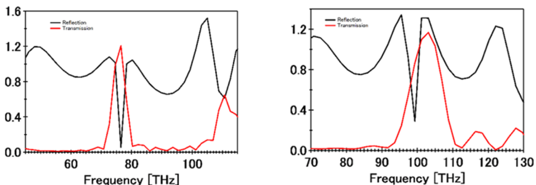
Figure 1 Electromagnetic field simulation of wavelength-selective infrared emitting devices with additional multilayer film structures. The results show tuning of the emission wavelength by different film thicknesses.
