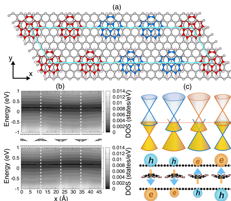
Fig. 1 (a) A geometric structure of superlattice consisting of strips of bilayer graphene where corannulene is alternately arranged in convex and concave with quadruple periodicity. Red, blue, gray, and pink balls denote C atoms of corannulene molecule with convex arrangement, C atoms of corannulene molecule with concave arrangement, C atoms of bilayer graphene, and H atoms, respectively. Right blue lines indicate a unit cell. (b) pDOS of corannulene-intercalated bilayer graphene on C atoms belonging to the upper layer and lower layer. (c) A schematic band diagram associated with the Dirac points near the interface between corannulene with convex and concave arrangements in bilayer graphene.
