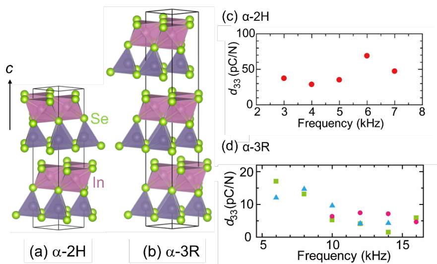
Figure 1 Piezoelectric effect in 2H and 3R phases of \alpha - \text{In}_2\text{Se}_3 . (a,b) Crystal structure of \alpha - \text{In}_2\text{Se}_3 in (a) 2H and (b) 3R phases. (c,d) Piezoelectric d_{33} coefficient as a function of measurement frequency for (c) 2H and (d) 3R samples. Larger d_{33} values are observed for the 2H sample.
