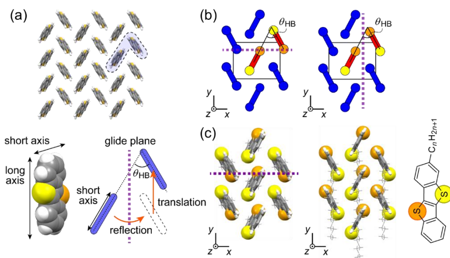
Figure 1 (a) (top) Layered herringbone (LHB)-type molecular packing. (bottom) Schematic illustration of the T-shaped molecular contact. The T-shape contacts are characterized by glide reflection symmetry. (b) Schematic representations of distinct glide symmetries in LHB polymorphs. The glide planes are perpendicular to the y-axis and x-axis, as indicated by the purple dotted lines. (c) Molecular packing structures of mono- C_n -BTBTs. The left and right panels show short-chain and long-chain type polymorphs, respectively.
