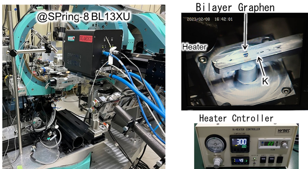
Figure 1 Photograph of experimental setup for in-situ X-ray diffraction experiment of K intercalation of bilayer graphene.
