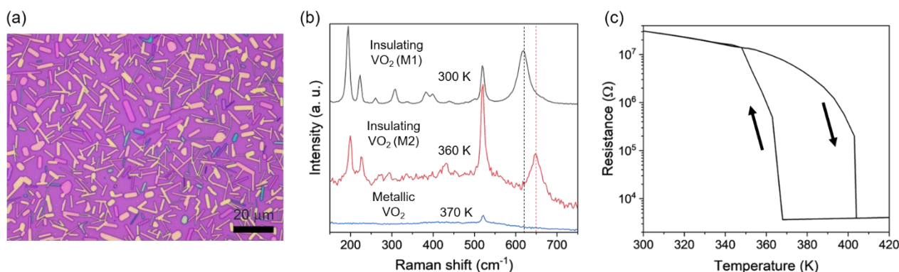
Figure 1 (a) Optical image of \text{VO}_2 grown by CVD on a \text{Si}/\text{SiO}_2 substrate. (b) Raman spectra of CVD-grown \text{VO}_2 at 300, 360, and 370 K. (c) Resistance-temperature curves of CVD-grown \text{VO}_2 . The arrows indicate the directions of the temperature sweep.
