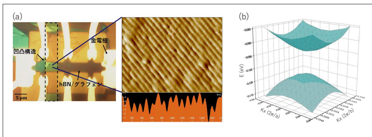
Figure 1 (a) Optical microscope image of the sample and AFM image of the line and space structure. (b) Calculated band structure of graphene with periodic strain (period 20 nm, strain 1%).
