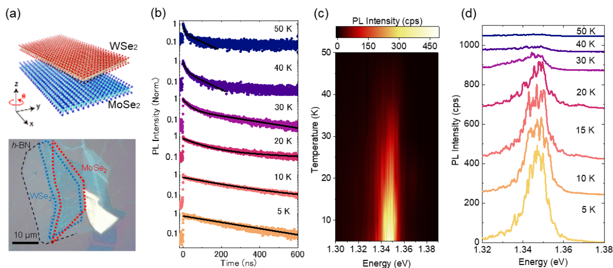
Figure 1 (a) Schematic of semiconducting \text{MoSe}_2/\text{WSe}_2 heterobilayer (upper part). Optical microscope image of \text{MoSe}_2/\text{WSe}_2 heterobilayer (lower part), (b) Photoluminescence (PL) decay profiles of moiré exciton as a function of temperature, (c) Temperature dependence of PL intensity, (d) Temperature dependence of PL spectra.
