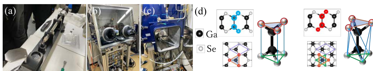
Figure 1 (a) Newly-developed double-tilt 4-electrodes air exposure preventing TEM sample holder for UHR pole piece from Mel-Build Corporation, (b) Glove box for setting TEM samples under Ar atmosphere and low humidity, (c) Pass box with the TEM sample holder inside, and (d) GaSe monolayer with conventional trigonal prismatic structure (left) and newly- discovered, metastable trigonal anti-prismatic structure (right).
