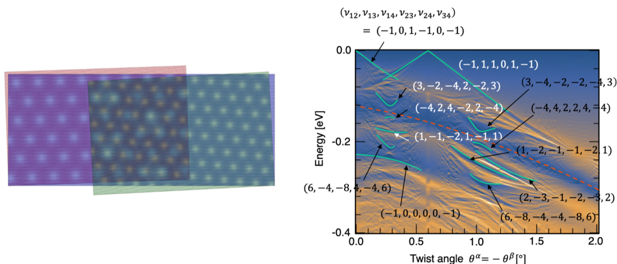
Figure 1 Moiré pattern in hBN/graphene/hBN trilayer system (left), and its electronic spectrum plotted against the relative twist angle (right).
