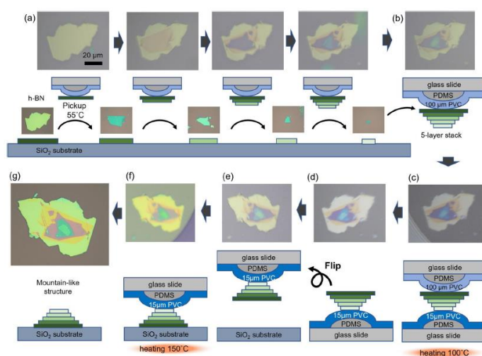
Figure 1 Demonstration of flip-over stacking. (a) Five h-BN flakes on a SiO 2 /Si substrate were picked up by a 100-μm-PVC/PDMS stamp at T = 55\text{ }^{\circ}\text{C} , starting with the largest and proceeding to sequentially smaller flakes, and hence (b) an inverse-mountain-like stacked structure was created. (c) The stack was brought into contact with and (d) transferred to a 15-μm-PVC/PDMS stamp at T = 100\text{ }^{\circ}\text{C} . (e) The 15-μm-PVC/PDMS stamp was inverted and (f) brought into contact with a SiO 2 /Si substrate before being slowly detached at T = 150\text{ }^{\circ}\text{C} . (g) The stack was dry-released on the substrate, and a mountain-like layered h-BN structure was obtained.
