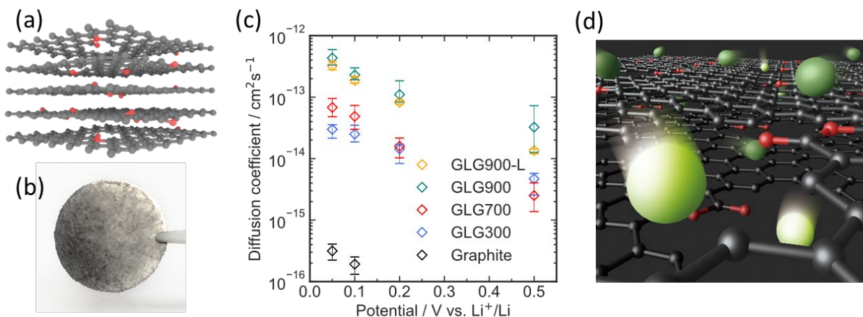
Figure 1 Synthesis of GLG sheet and elucidation of ion diffusion behaviors of it. (a) Structure model of GLG. (b) Photograph of GLG sheet. (c) Diffusion coefficient of graphite and GLGs at 0.05, 0.1, 0.2, and 0.5 V vs Li + /Li. Here, GLG900-L is prepared from GO synthesized at 0 °C and then heat treated at 900 °C. (d) Schematic illustration of the diffusion of lithium ions through nanopores in GLG.
