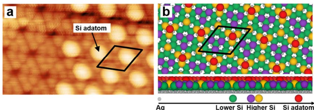
Figure 1 (a) AFM topographic image of silicene surface with additional Si adatoms. Imaging parameters: \Delta f = -12 Hz, V_S = 0.75 V, 3.8 \times 8.0 nm 2 , T = 78 K. (b) DFT optimized atomic structure of the silicene decorated with Si adatoms. Black rhombus indicates the unit cell of 2D island of Si adatom on silicene.
