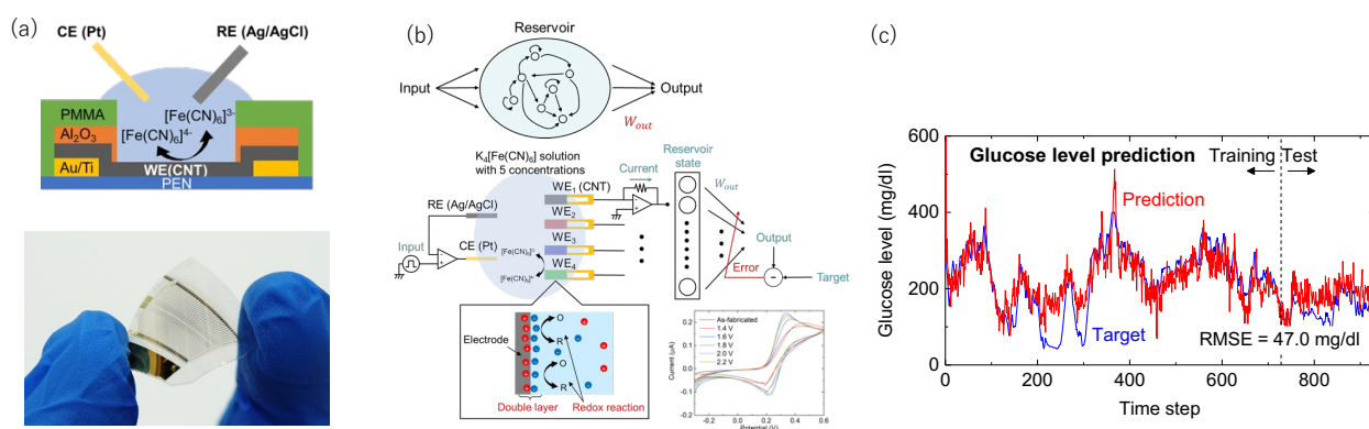
Figure 1 Reservoir computing based on carbon nanotube electrochemical sensors. (a) Schematic and photograph of carbon nanotube electrochemical sensor fabricated on plastic film. (b) Schematic of reservoir computing system based on carbon nanotube electrochemical sensor array. (c) Result of blood glucose level prediction task.
