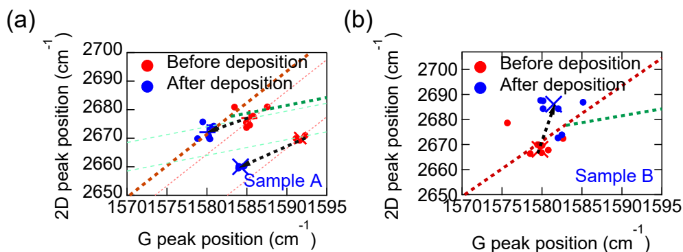
Figure 1 2D-G peak energy plots of the air suspended twisted bilayer graphene before (Red) and after (Blue) Ga metal deposition. Measurements were taken from several different holes of TEM grid. Figure (a) shows the plots for sample A composed of two CVD graphene and figure (b) shows that for sample B composed of both CVD and epitaxial graphene.
