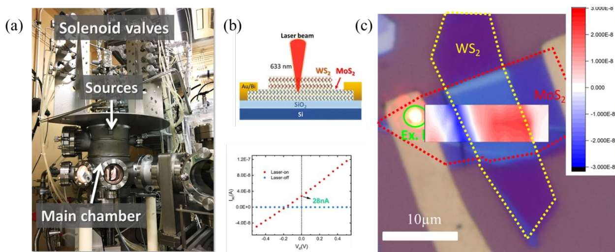
Figure 1 (a) Photograph of the MOCVD setup developed. Using this MOCVD setup, bilayer lateral heterostructures can be grown. (b) top: Schematic representation of a two-terminal device with a WS 2 /MoS 2 channel, and bottom: IV characteristic under laser excitation. (c) Optical image of the two-terminal device and a photocurrent mapping result measured at room temperature.
