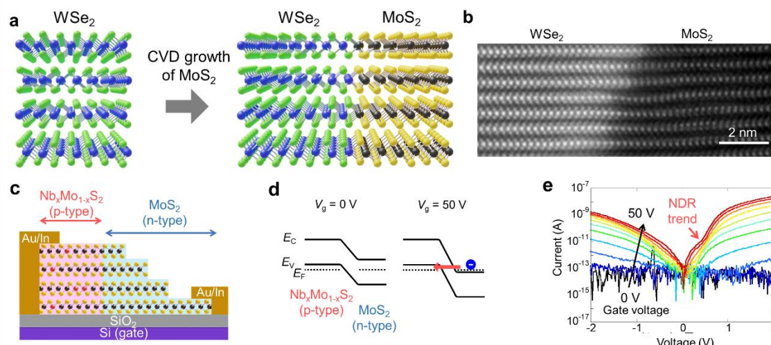
Figure 1 (a) Schematic of the growth process and (b) scanning transmission electron microscopy (STEM) image of an in-plane heterostructure of multilayer TMDCs. Schematics of (c) the device structure and (d) the band diagram of \text{Nb}_x\text{Mo}_{1-x}\text{S}_2 and \text{MoS}_2 in-plane heterostructure. (e) Current-voltage curves as a function of gate voltage.
