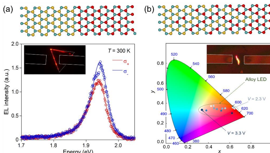
Figure 1 Monolayer in-plane heterostructure light-emitting devices. (a) Schematic, EL image, and EL spectrum obtained from \text{WS}_2/\text{WSe}_2 steep heterojunction interfaces. (b) Continuous color-tunable light-emitting devices based on compositionally graded interfaces of \text{WS}_2/\text{WSe}_2 alloys.
