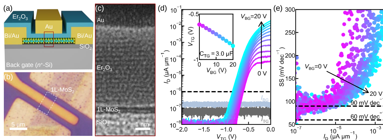
Figure 1 (a,b) Top-gated monolayer MoS 2 FET using a thermally-evaporated Er 2 O 3 as the gate dielectric. (c) Cross-sectional TEM image of the top gate stack. (d) Bidirectional transfer characteristics at constant V_D = 2 V, various V_{BG} = 0 –20 V. Inset: V_{TG} at I_D = 10^{-6} μA/μm as a function of V_{BG} . The slope of the linear fit yields the ratio of the top and bottom oxide capacitance, thus the extraction of C_{TG} was achieved. (e) Subthreshold swing as a function of I_D at different V_{BG} .
