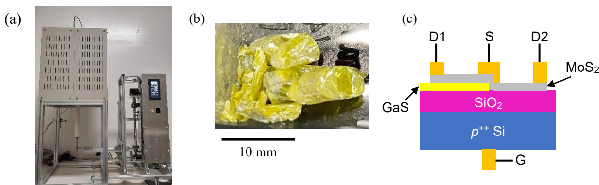
Figure 1 (a) Single-crystal growth system by the Bridgman method. (b) GaS single crystals grown by the Bridgeman method. (c) Schematic diagram of a MoS 2 field-effect transistor with GaS as a buffer layer.
