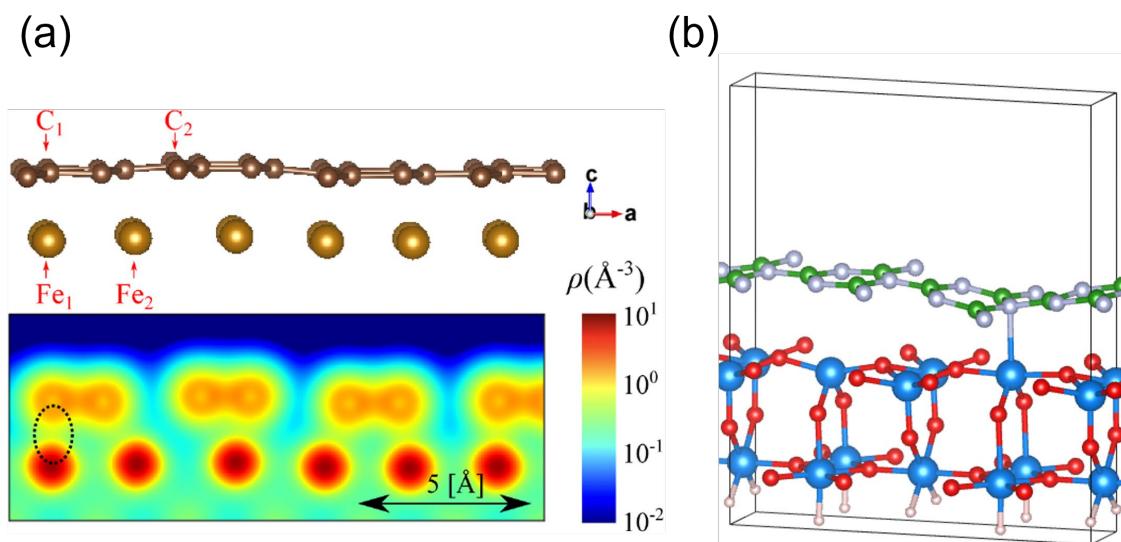
Figure 1 (a) Charge density profile of the FePd(001)/Gr interface. C 1 and Fe 1 represent the closest pair, and C 2 and Fe 2 are examples of sites with no close C or Fe atoms. Reprinted from M. Uemoto et al. , J. Appl. Phys. , 132 , 095301 (2022). (b) Atomic structure of VO 2 /h-BN interface. Blue, red, white, gray, green balls are V, O, H, N, and B atoms, respectively.
