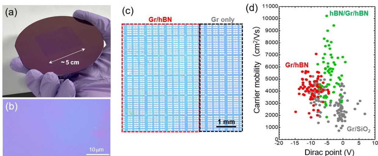
Figure 1 CVD synthesis of multilayer hBN and the integration with CVD-grown monolayer graphene. (a,b) Photograph and optical images of large-area, multilayer hBN. (c) Device arrays of graphene/hBN and graphene channels. (d) Comparison of the carrier mobility of different types of graphene devices.
