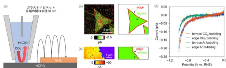
Fig. 1 (a) A schematic illustration of SECCM imaging. (b) HER imaging on MoS 2 nanosheet. (c) CO 2 RR imaging on SnS 2 nanosheet. (d) cyclic voltammetry of edge and terrace of SnS 2 nanosheet.
