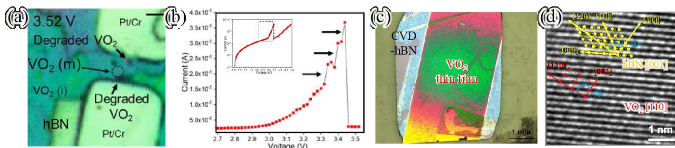
Figure 1 Optical microscope image of \text{VO}_2 film on single crystalline h-BN flake for current induced resistive switching device, (b) Voltage – Current characteristic of \text{VO}_2/\text{crystalline h-BN} flake device, (c) Optical microscope image of pulsed laser deposition grown \text{VO}_2 film on CVD-grown h-BN film, (d) Plane view TEM image of \text{VO}_2 film on CVD-grown h-BN.
