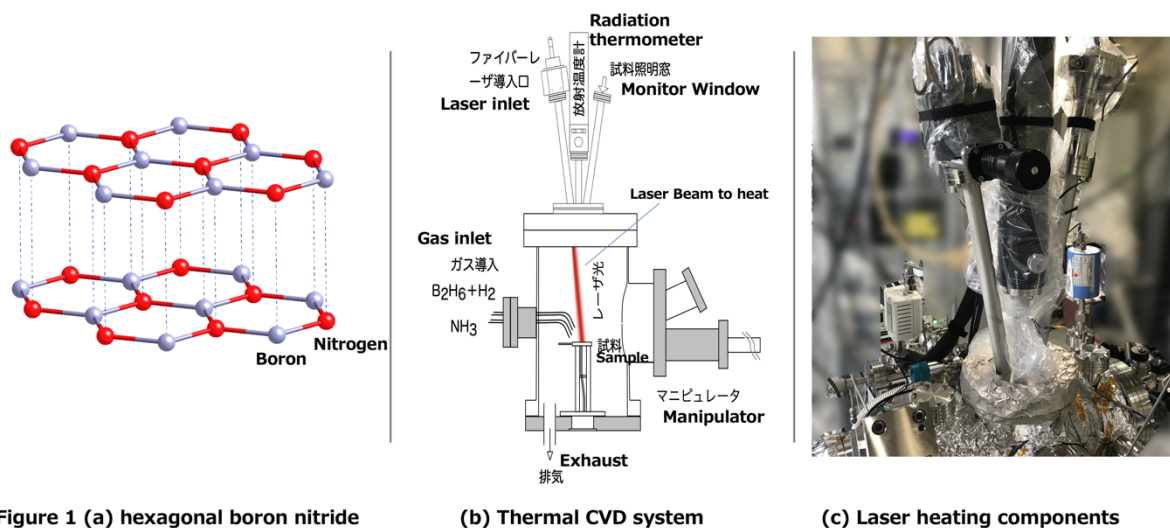
Figure 1 (a) hexagonal boron nitride (b) Thermal CVD system (c) Laser heating components Figure 1 (a) Crystal structure of hexagonal boron nitride, (b) and (c) Schematics of Laser heated thermal CVD system for hBN growth.
