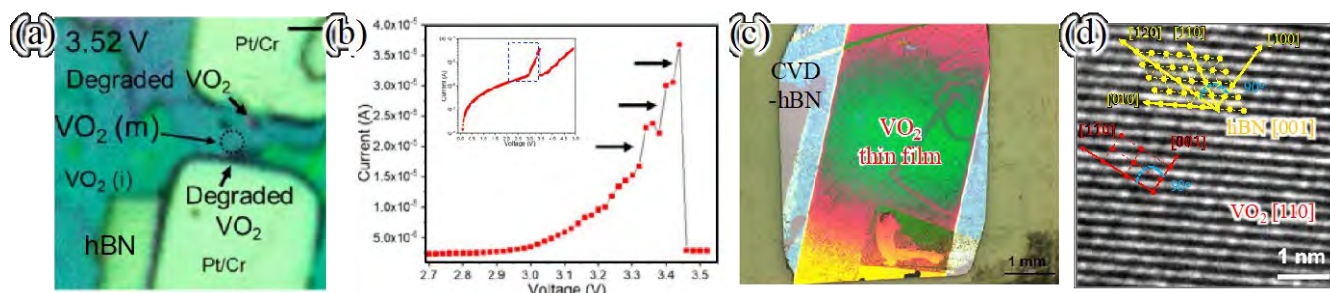
Figure 1 Optical microscope image of \text{VO}_2 film on single crystalline h-BN flake for current induced resistive switching device, (b) Voltage – Current characteristic of \text{VO}_2 /crystalline h-BN flake device, (c) Optical microscope image of pulsed laser deposition grown \text{VO}_2 film on CVD-grown h-BN film, (d) Plane view TEM image of \text{VO}_2 film on CVD-grown h-BN.
