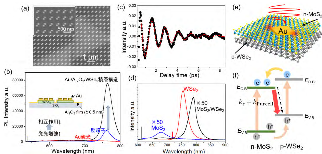
Figure 1 (a) SEM image of Au/Al 2 O 3 /WSe 2 nanostructures. (b) PL enhancement of Au/Al 2 O 3 /WSe 2 nanostructures. (c) Coherent optical phonon signals of interlayer breathing mode of bilayer WSe 2 . (d) PL spectra of MoS 2 /WSe 2 heterostructure, WSe 2 and MoS 2 . (e) A schematic illustration of plasmon-enhanced light energy conversion devices using Au nanostructured TMDC heterostructure. (f) Energy diagram of plasmon-enhanced electroluminescence device using TMDC heterostructure.
