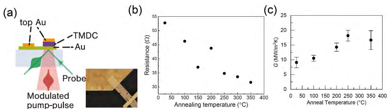
Figure 1 Schematic illustration of experimental setups for thermal and charge transport measurements across vdW interfaces formed by four layered MoS 2 samples. (b) Resistance and (c) thermal conductance as a function of annealing temperature.
