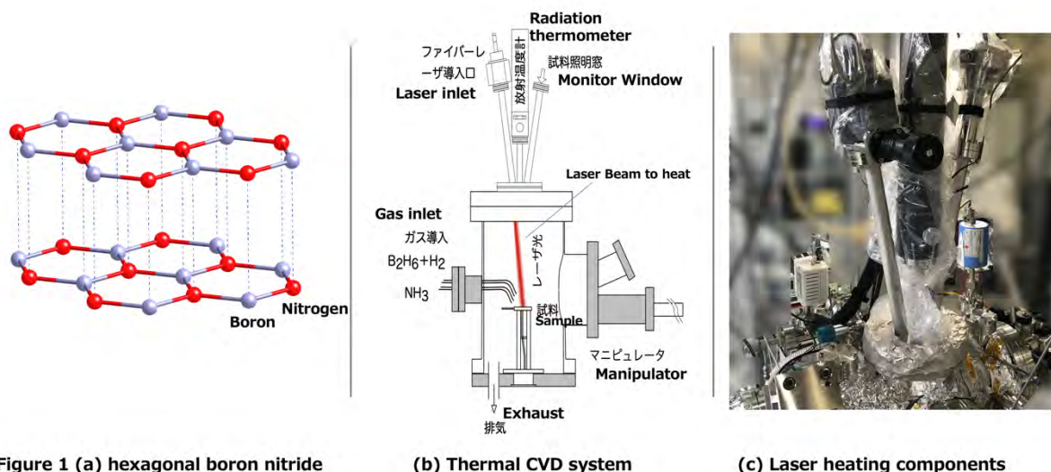
Figure 1 (a) Crystal structure of hexagonal boron nitride, (b ) and (c) Schematics of Laser heated thermal CVD system for hBN growth.
